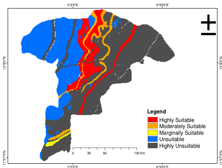
Figure 6: Reclassified rock types based on suitability
